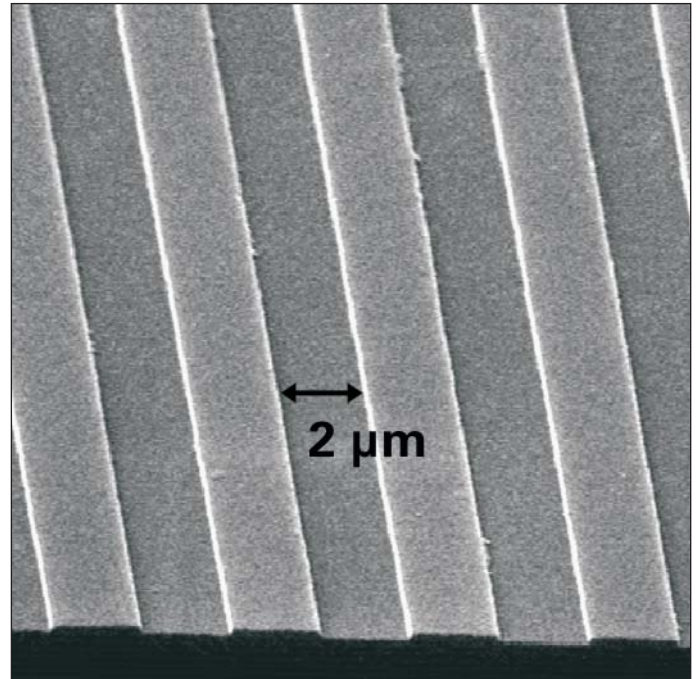
DIADUR phase grating with approx. 0.25\ \mu\text{m} grating height
